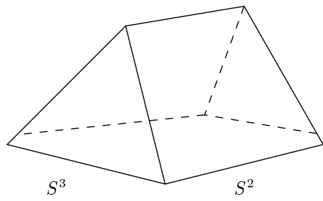
resolved conifold
