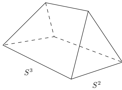
deformed conifold
