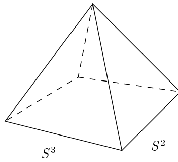
conifold
